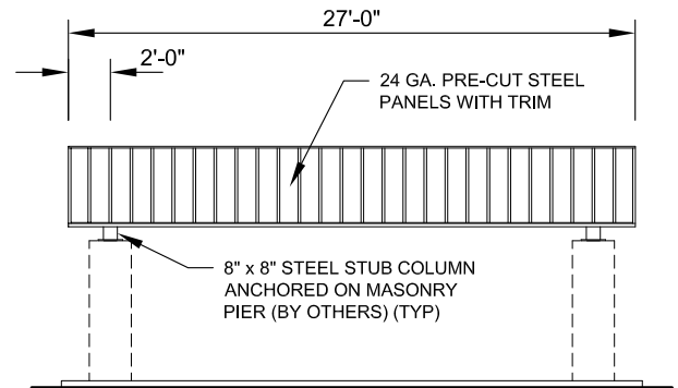
SIDE ELEVATION SCALE: NTS
