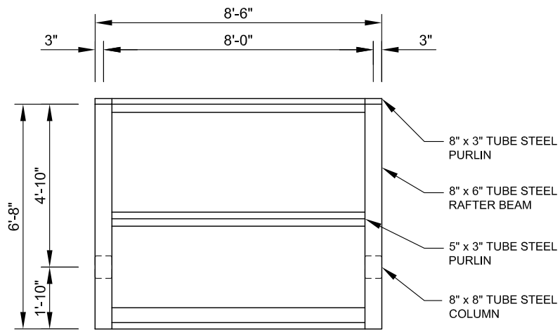
FRAMING PLAN SCALE: 1/4" = 1'-0"
