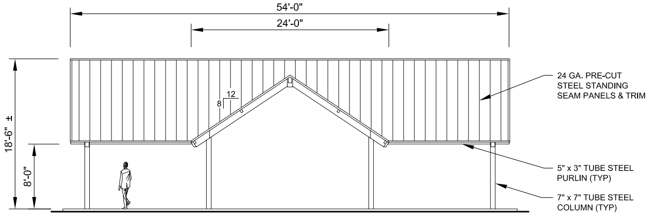
FRONT ELEVATION
