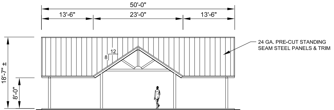
FRONT ELEVATION SCALE: NTS
