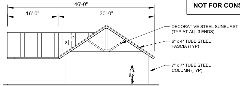
SIDE ELEVATION SCALE: NTS
