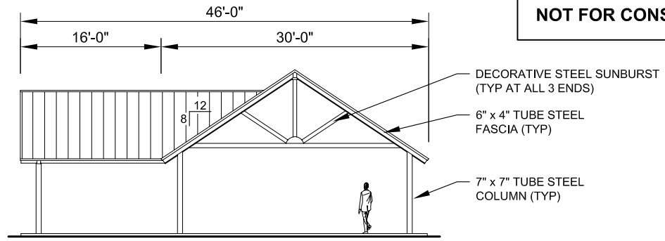
SIDE ELEVATION
