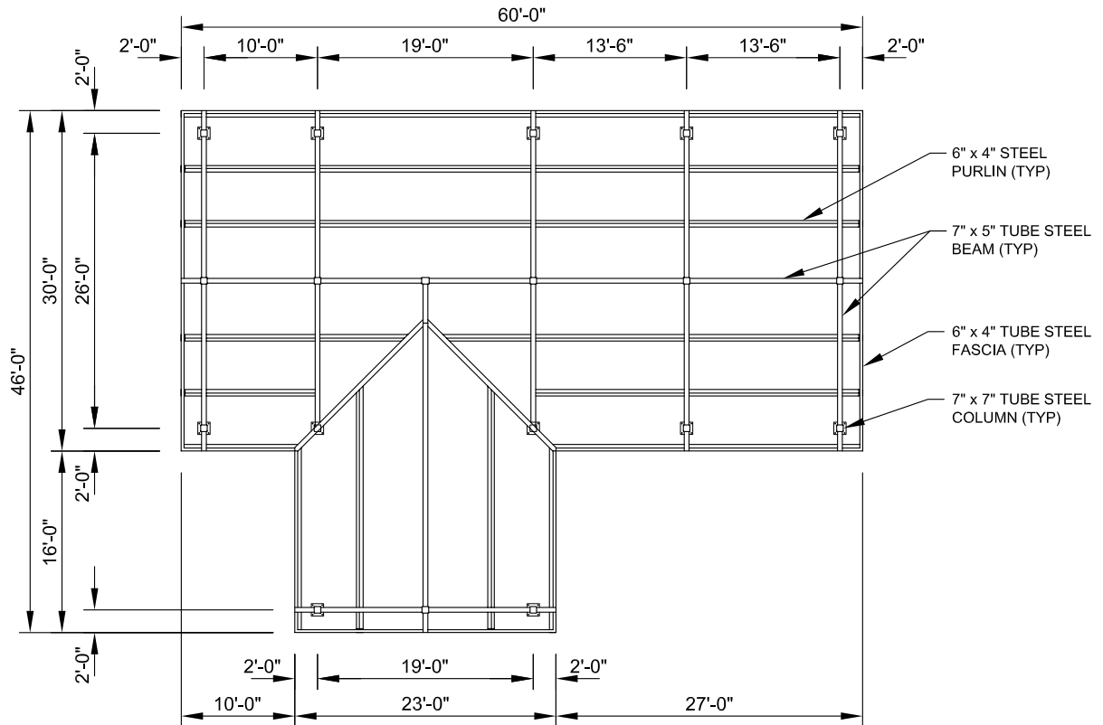
FRAMING PLAN
