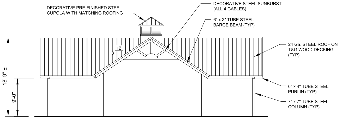
TYPICAL ELEVATION SCALE: NTS
