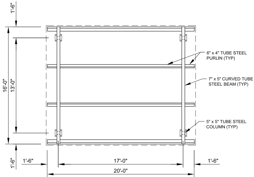
FRAMING PLAN SCALE: NTS
