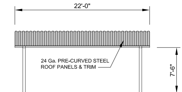
SIDE ELEVATION SCALE: NTS
