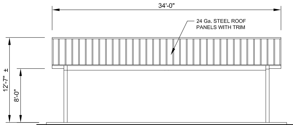
SIDE ELEVATION SCALE: NTS
