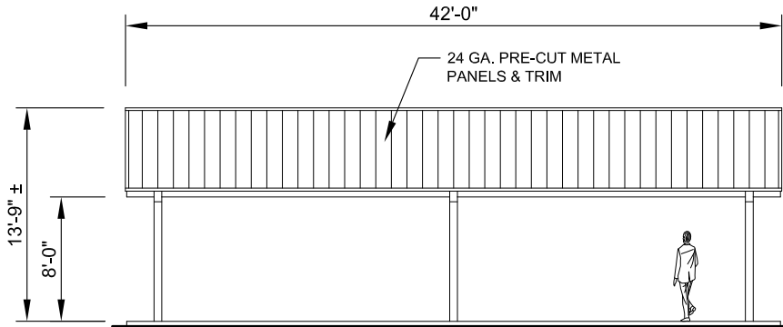
SIDE ELEVATION
