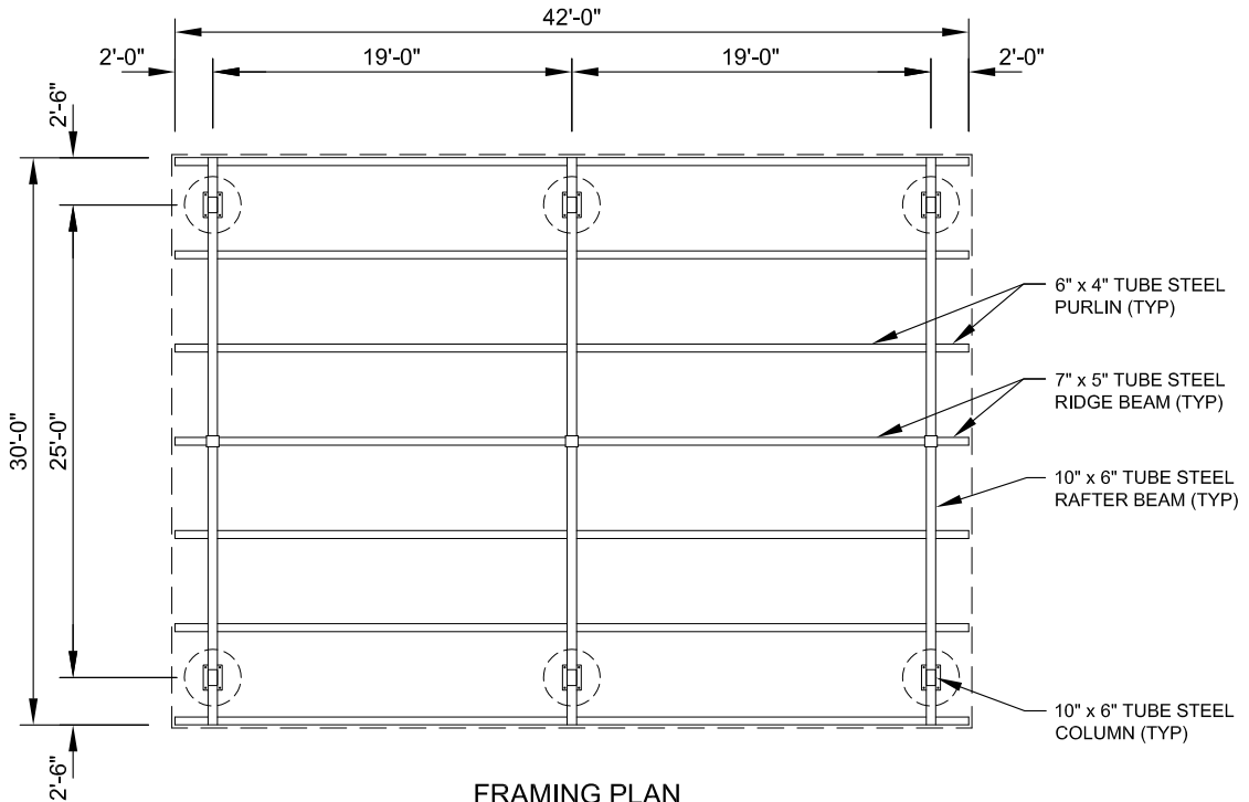
FRAMING PLAN
