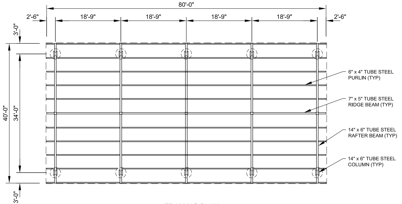
FRAMING PLAN SCALE: NTS
