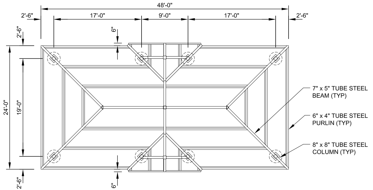
FRAMING PLAN
