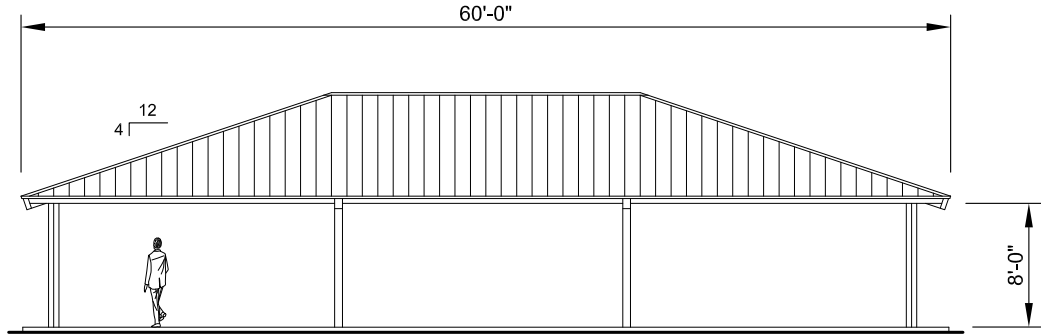
SIDE ELEVATION SCALE: NTS
