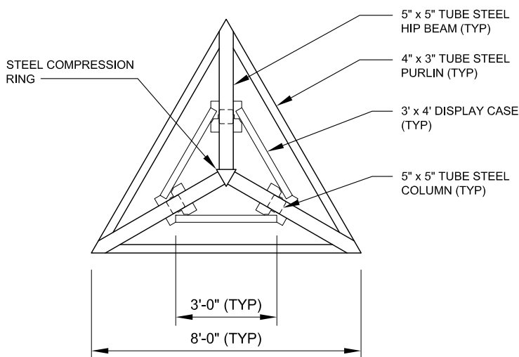
FRAMING PLAN SCALE: 1/4" = 1'-0"
