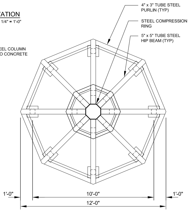
FRAMING PLAN SCALE: 1/4" = 1'-0"
