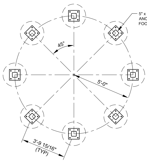
FOOTING LAYOUT SCALE: 1/4" = 1'-0"
