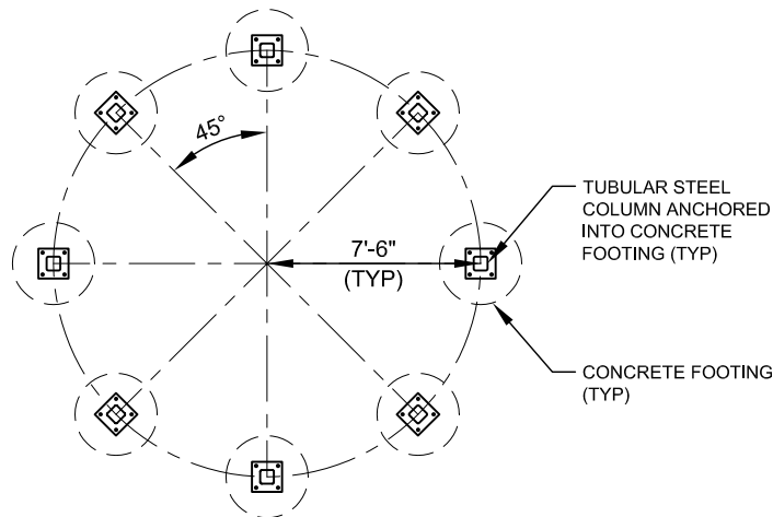
FOOTING LAYOUT PLAN SCALE: NTS
