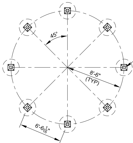
FOOTING LAYOUT PLAN
