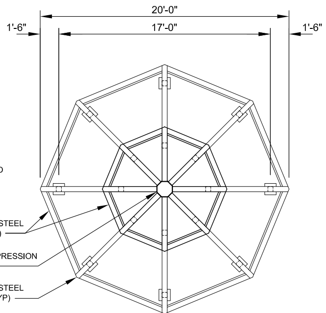
FRAMING PLAN
