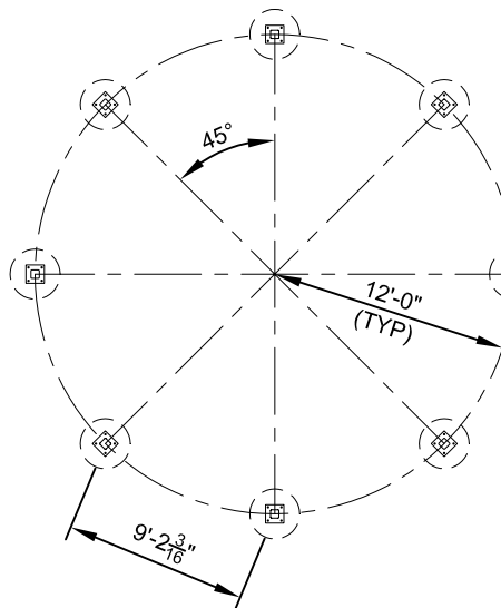
FOOTING LAYOUT PLAN SCALE: NTS
