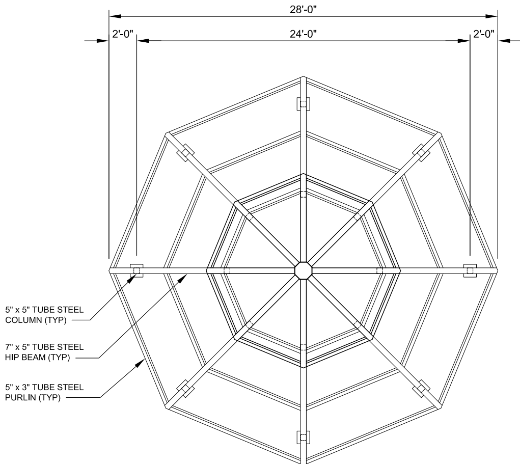
FRAMING PLAN SCALE: NTS
