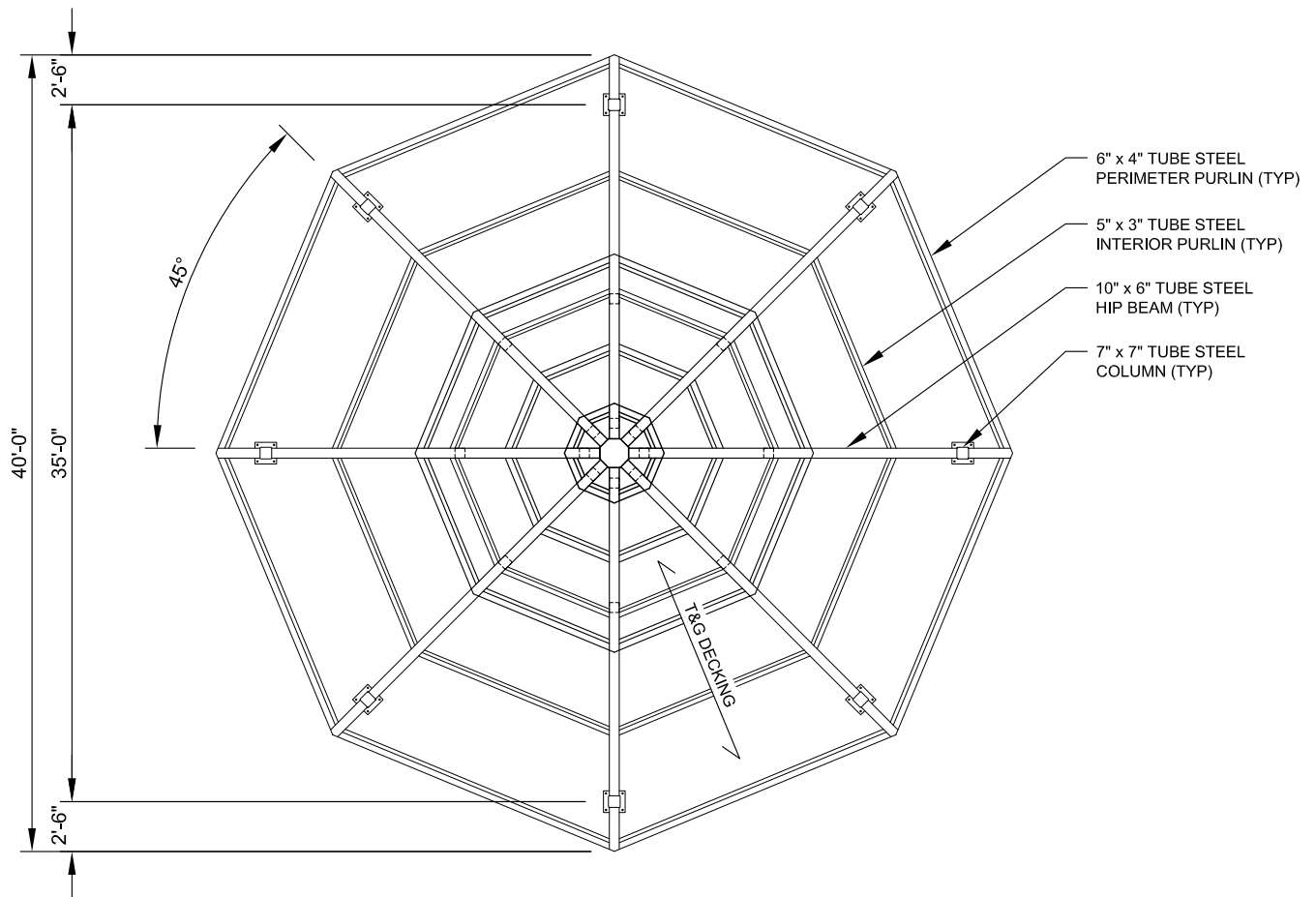
FRAMING PLAN SCALE: NTS
