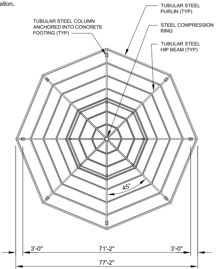
FRAMING PLAN SCALE: NTS
