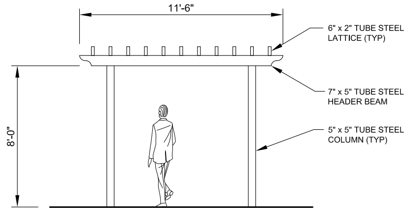
FRONT ELEVATION SCALE: NTS
