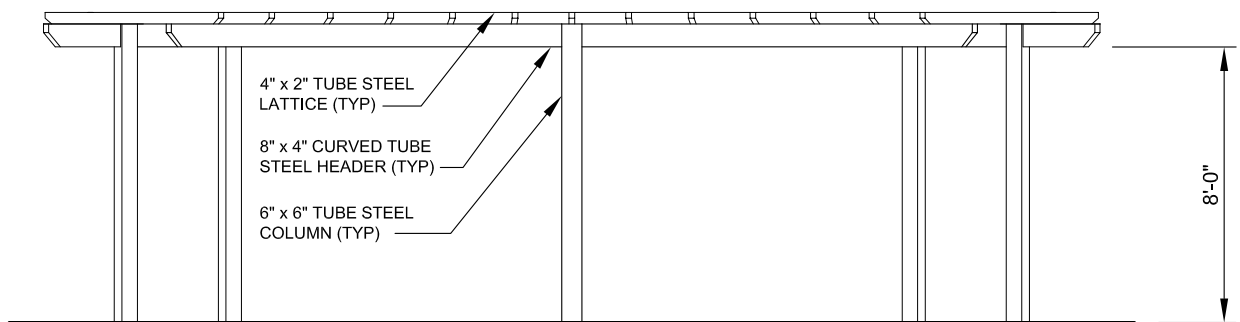
SIDE ELEVATION
