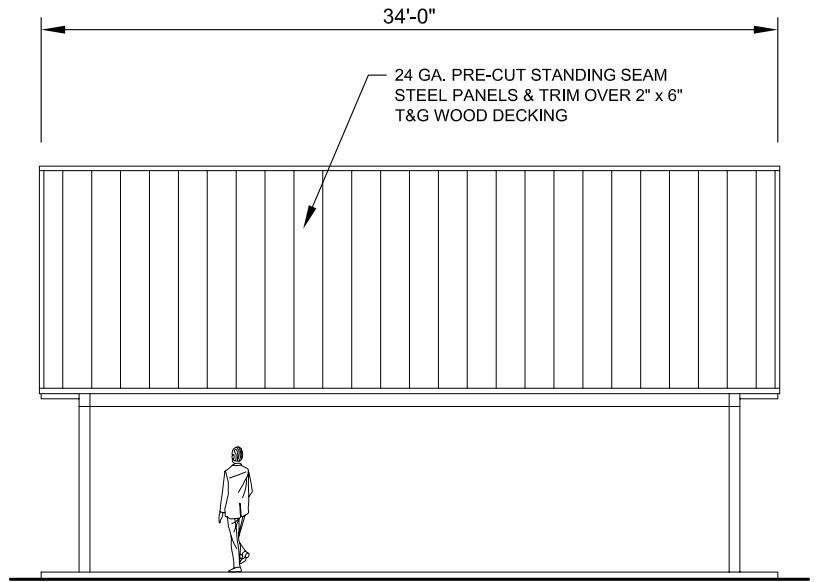
SIDE ELEVATION SCALE: NTS
