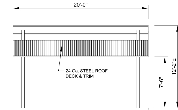
SIDE ELEVATION SCALE: NTS
