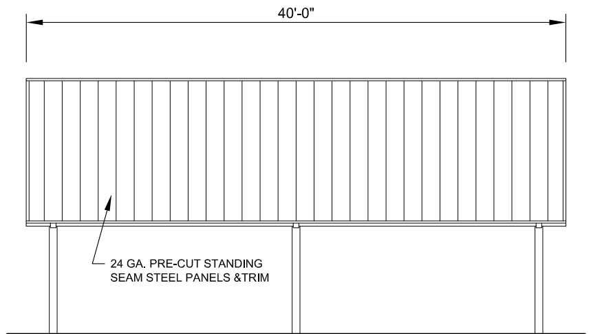
FRONT ELEVATION SCALE: NTS
