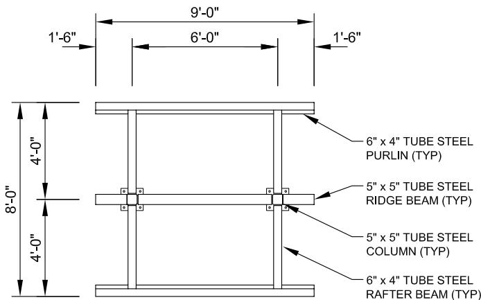
FRAMING PLAN SCALE: NTS
