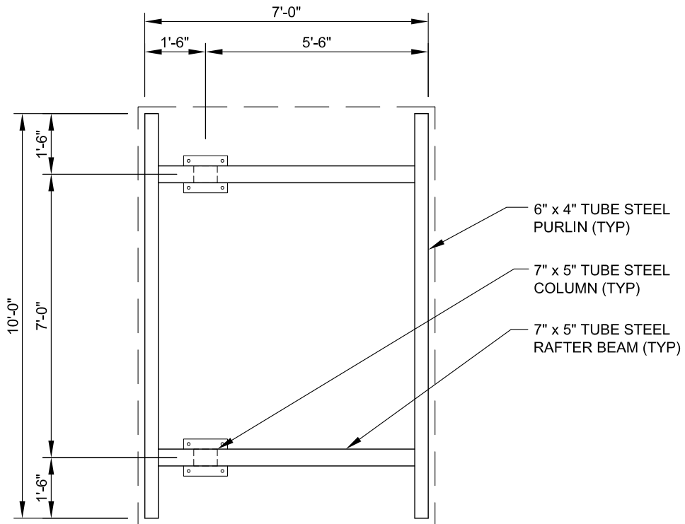
FRAMING PLAN
