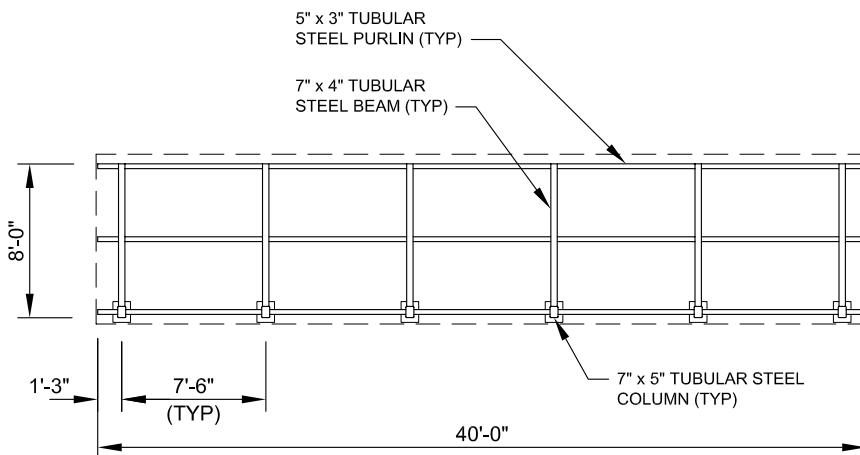
FRAMING PLAN
