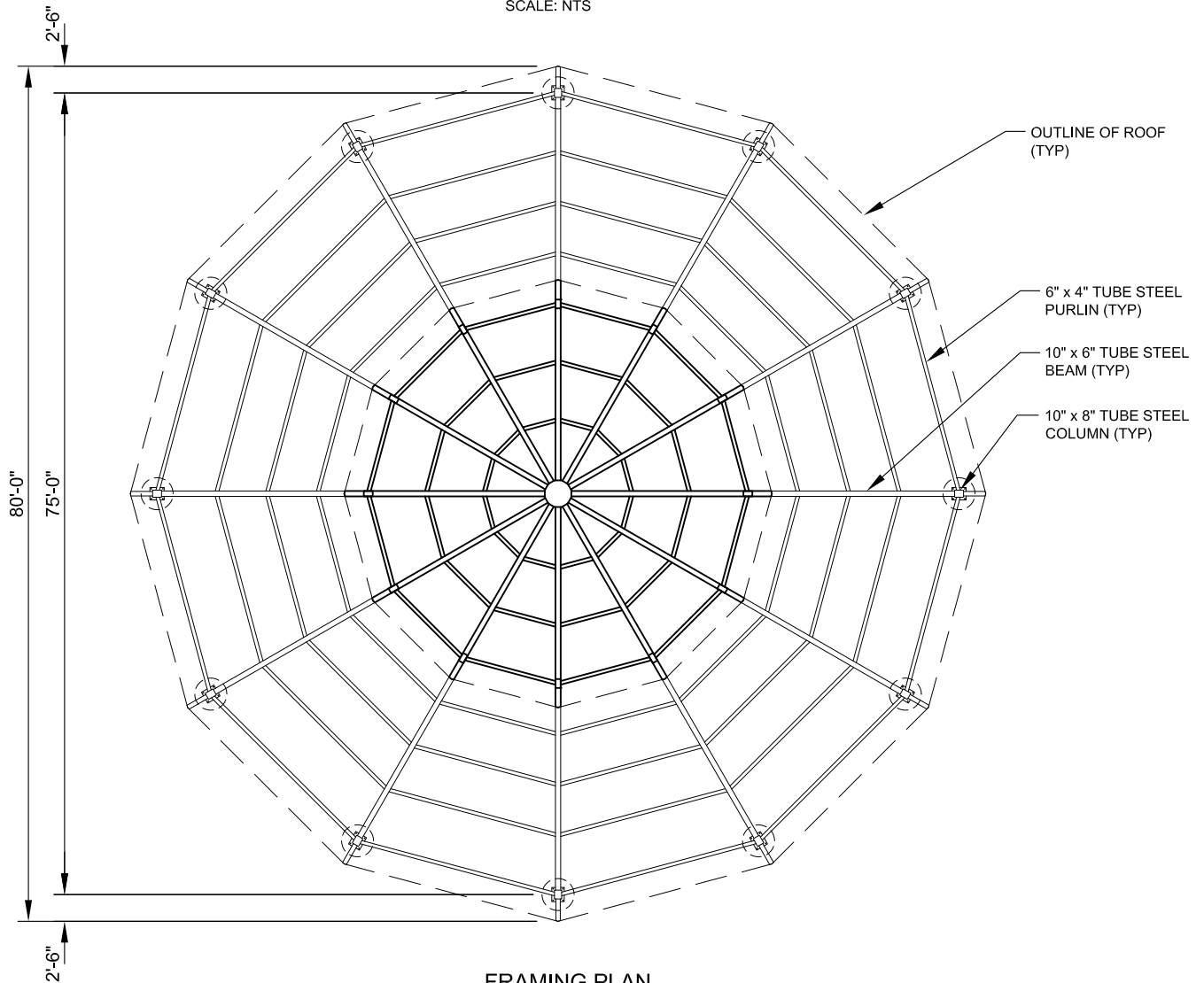
FRAMING PLAN
