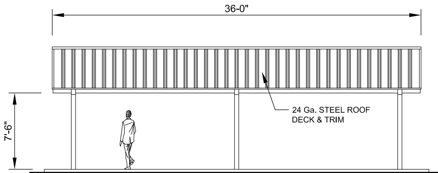
SIDE ELEVATION
