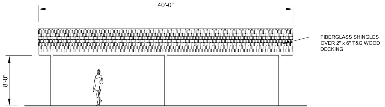
SIDE ELEVATION
