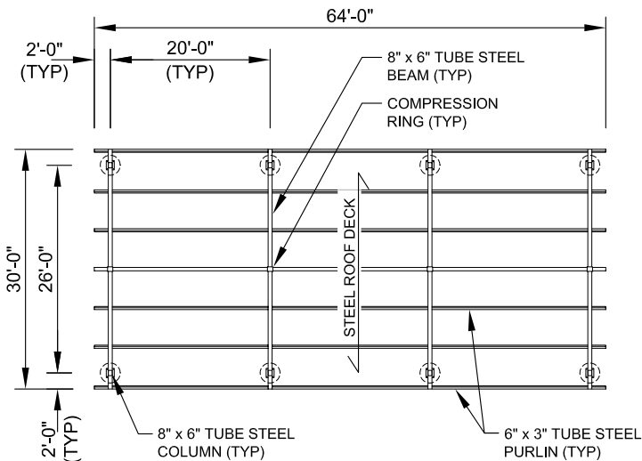
FRAMING PLAN
