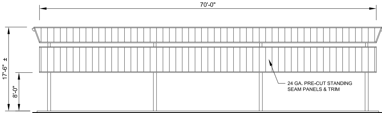
FRONT ELEVATION SCALE: NTS
