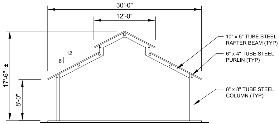
SIDE ELEVATION SCALE: NTS
