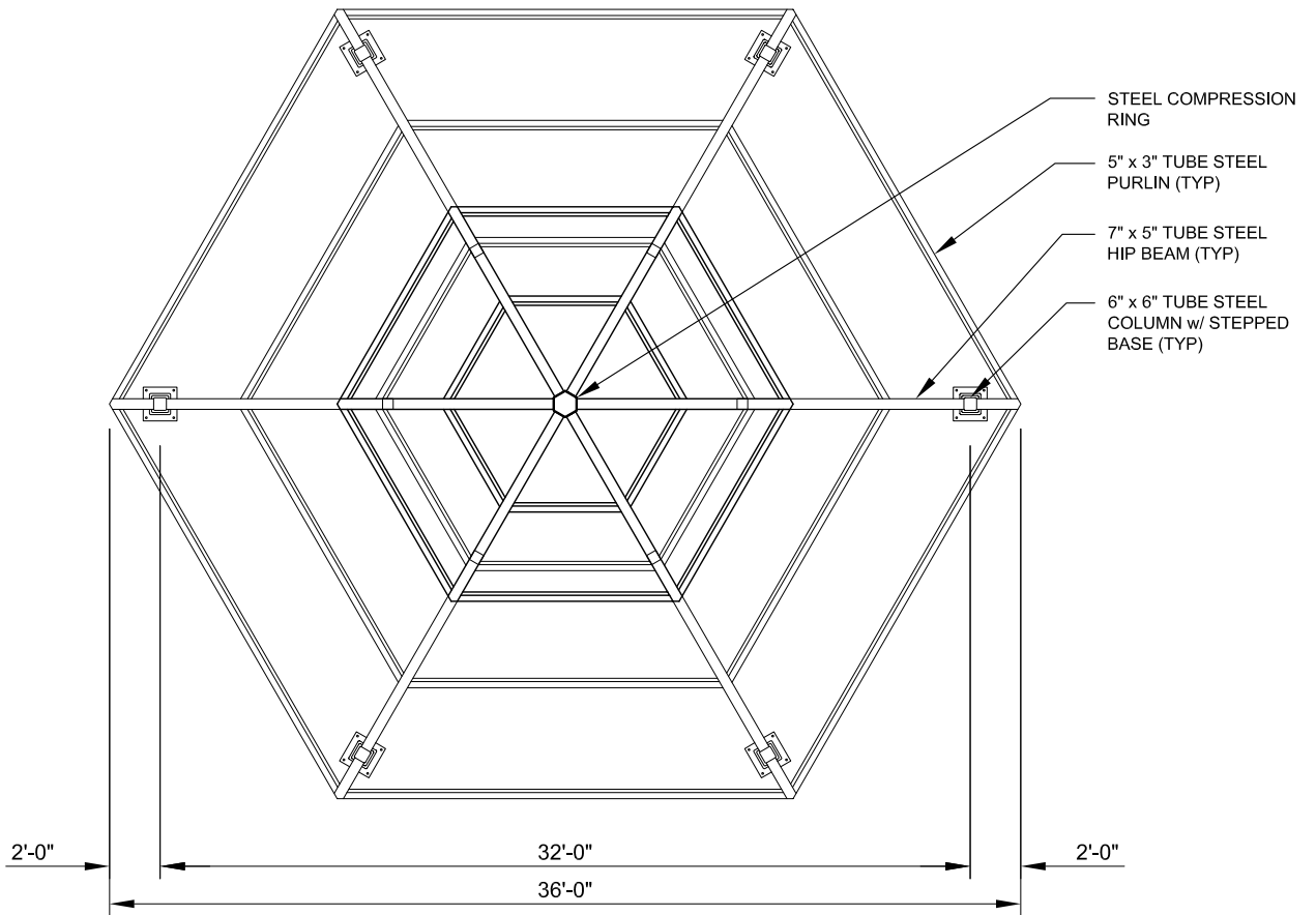
FRAMING PLAN SCALE: NTS
