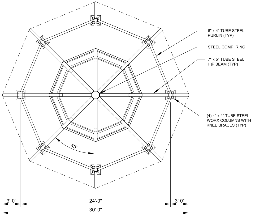
FRAMING PLAN SCALE: NTS
