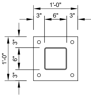
BASE PLATE DETAIL
