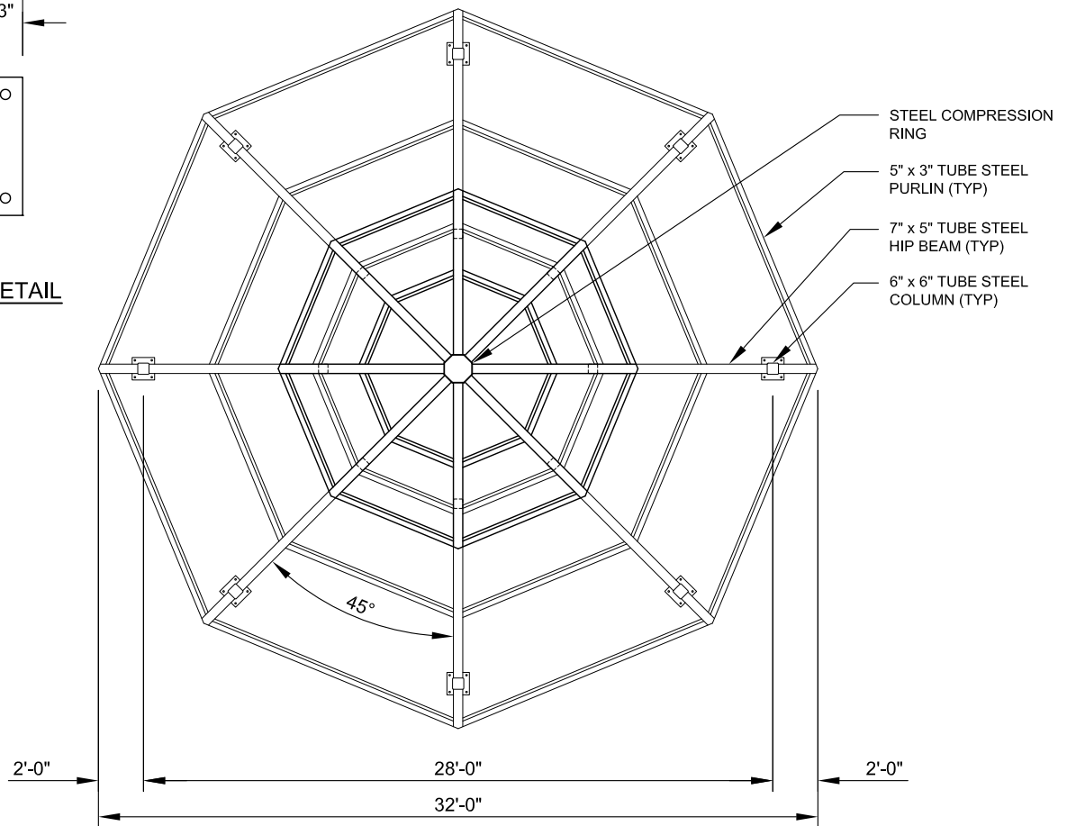
FRAMING PLAN
