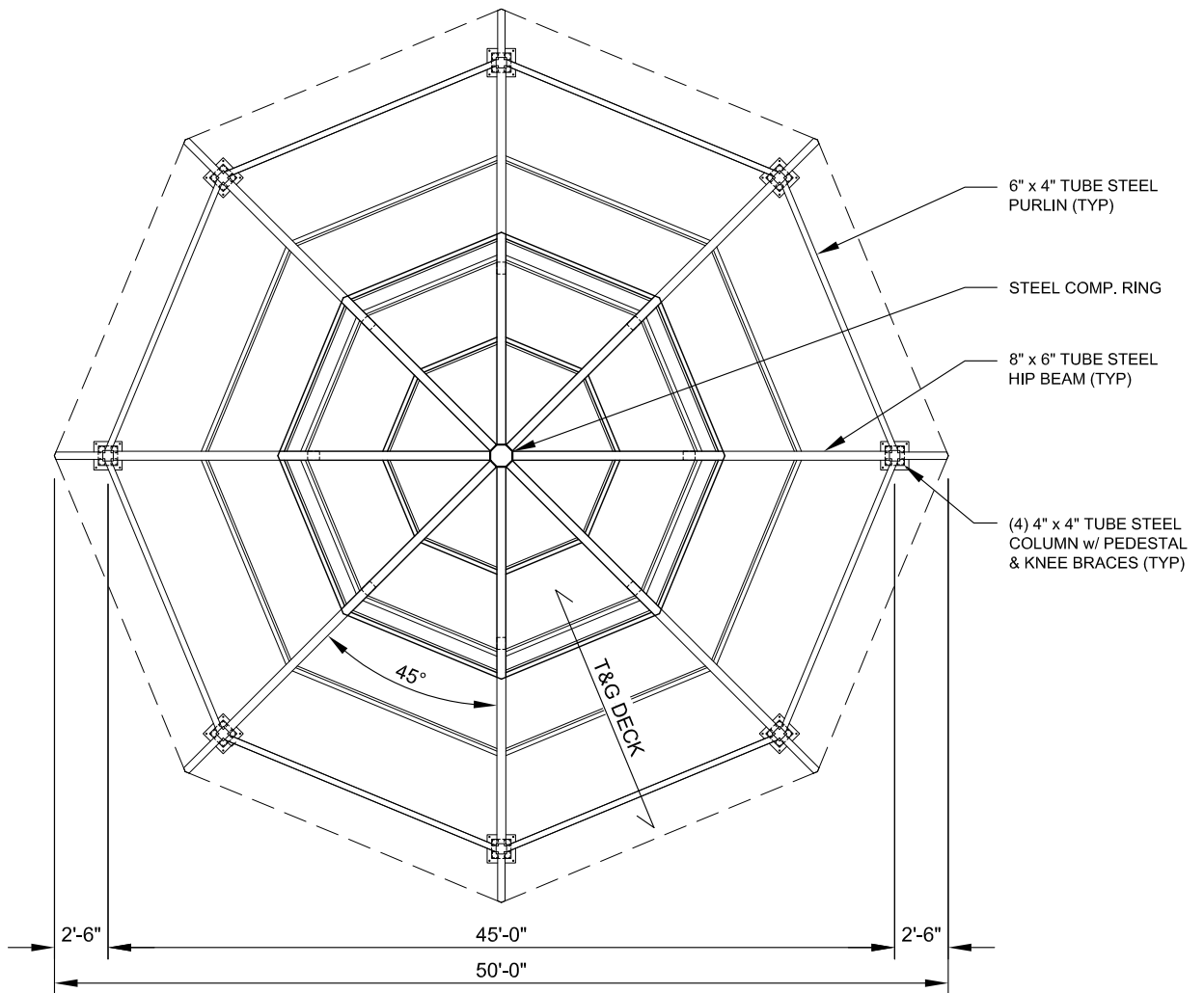
FRAMING PLAN SCALE: NTS
