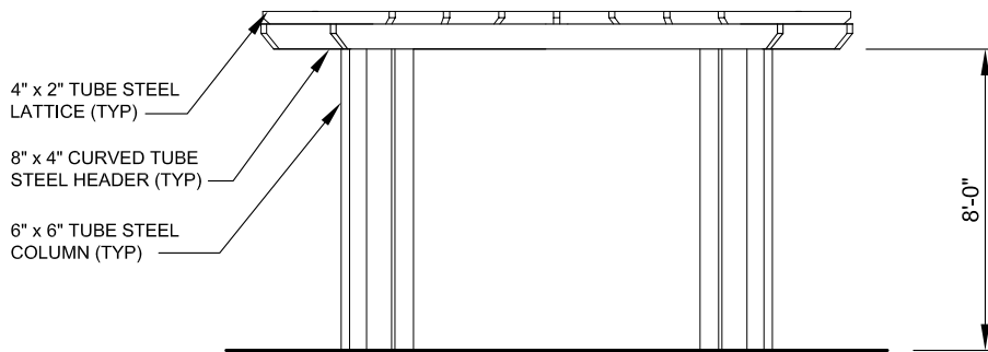
SIDE ELEVATION SCALE: NTS
