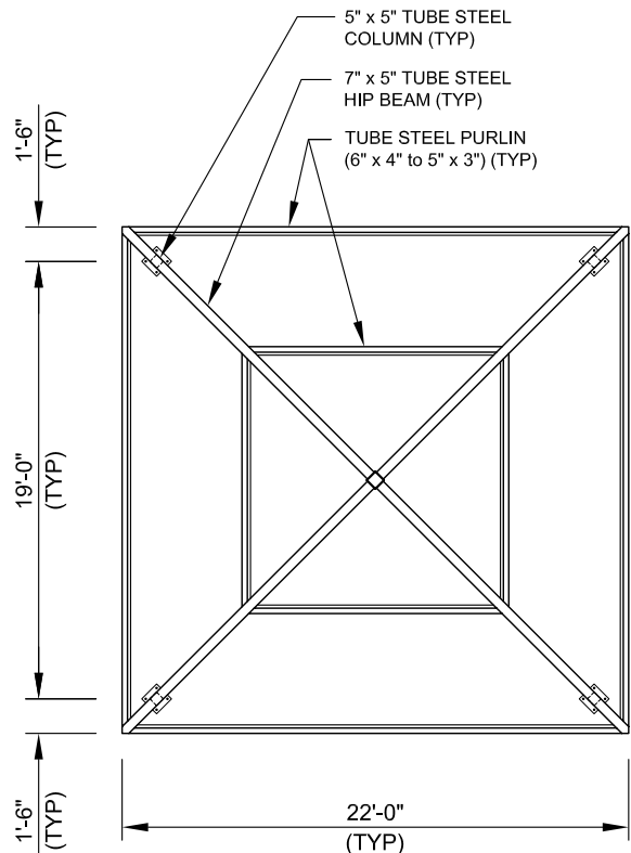
FRAMING PLAN SCALE: NTS
