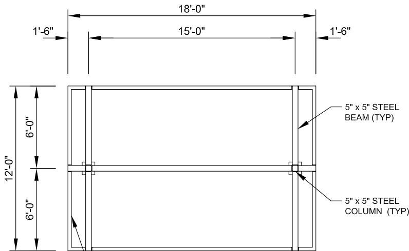
FRAMING PLAN
