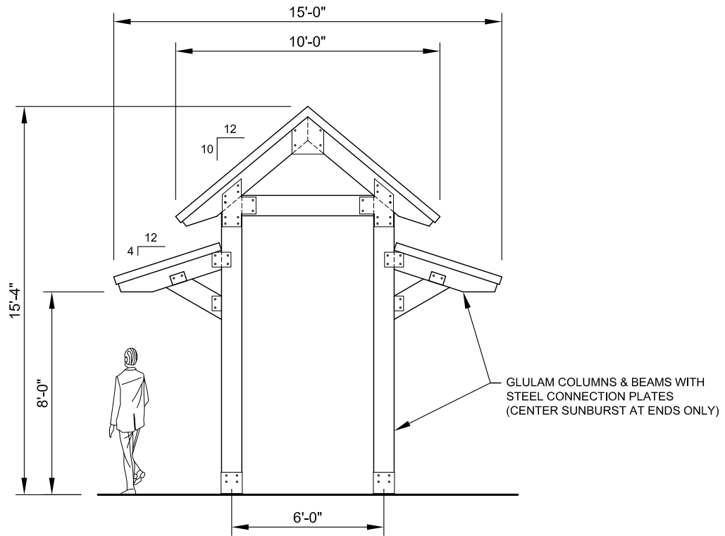
FRONT ELEVATION SCALE: NTS
